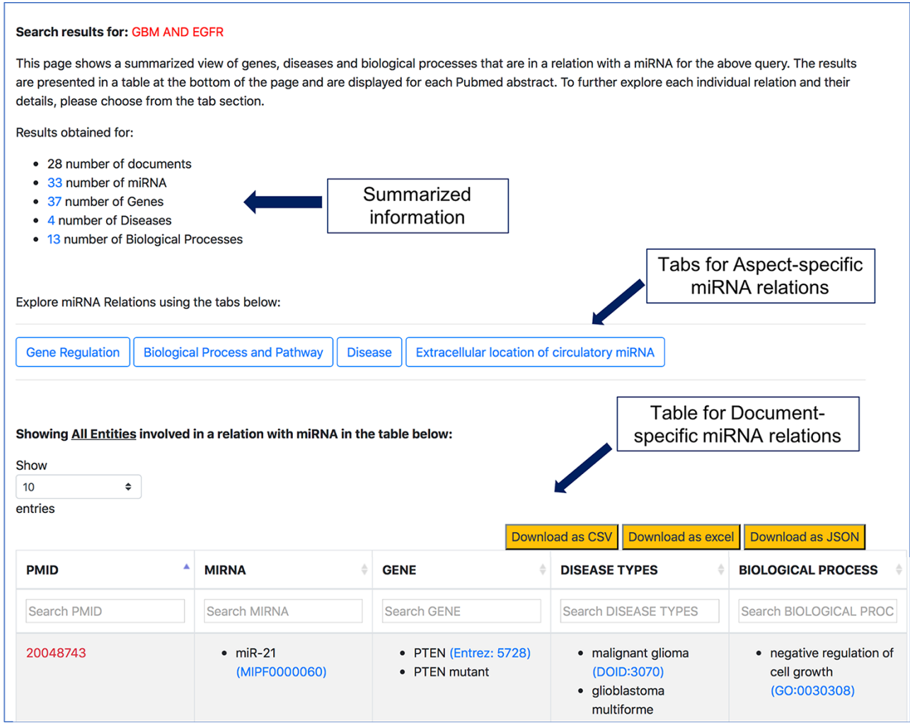
Figure 5. Screenshot of response page for context-centric query ‘GBM AND EGFR’.
