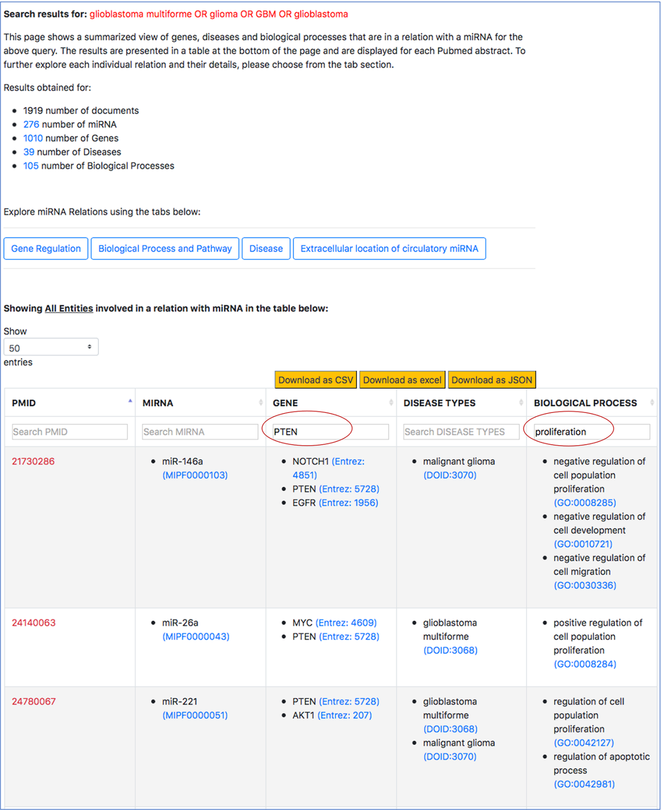
Figure 10. Filtered search result for 'PTEN' in the context of cell proliferation in GBM.
