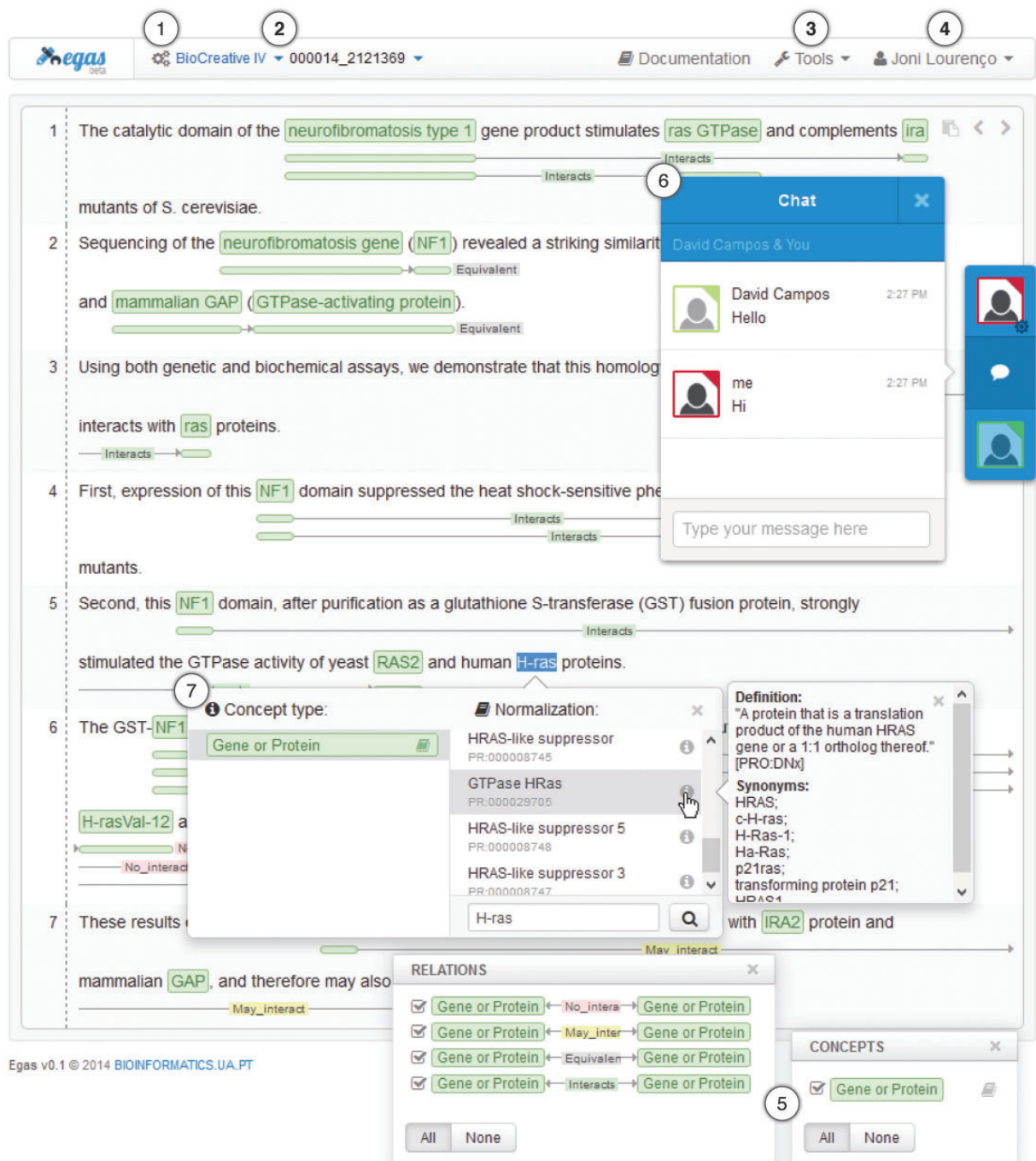
Figure 3. Egas main interface presenting a PubMed abstract (PMID 2121369) with annotated concepts and relations and emphasizing relevant interaction components/features: (1) project management; (2) project and document navigators; (3) processing tools; (4) account management; (5) concept and relation type visualization filters; (6) real-time collaboration; and, (7) concept annotation with normalization.
