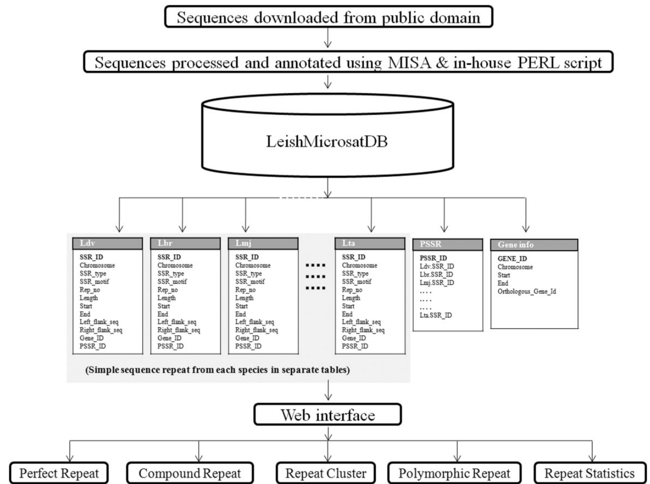
Figure 2. Architecture and data flow representation in LeishMicrosatDB.
