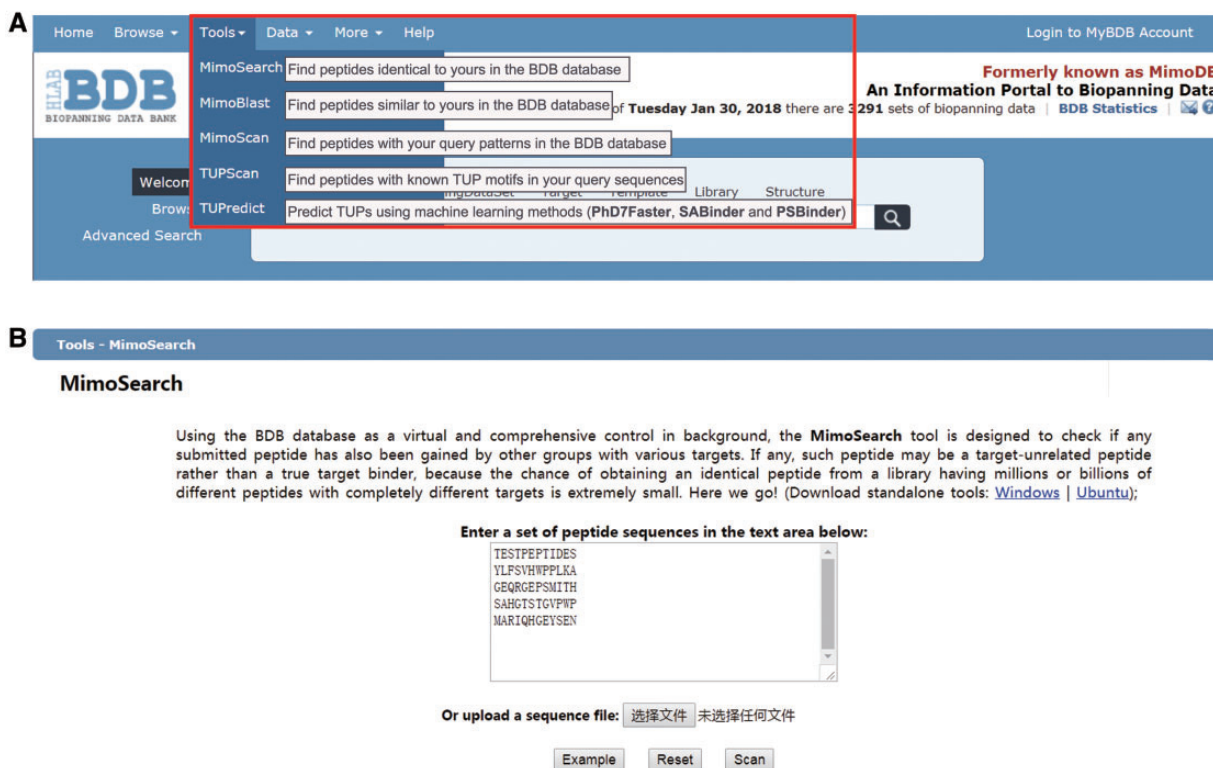
Figure 5. BDB-powered tools. (A) Seven tools surrounded by a red box, i.e. MimoSearch, MimoBlast, MimoScan, TUPScan, PhD7Faster, SABinder and PSBinder, can be accessible by clicking the secondary menu items from the 'Tools' drop-down menu. (B) We take MimoSearch as an example to show the utilization of these tools. Users can enter a set of peptide sequences in the text area or upload a sequence file. After submission, the result will be returned and displayed in a table.
