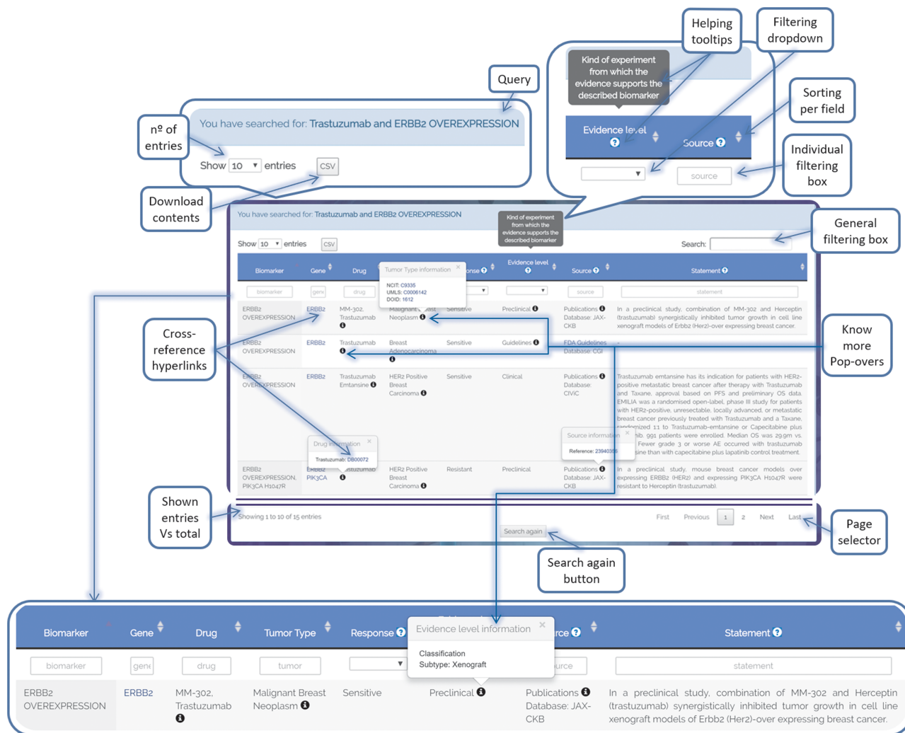
Figure 6. ResMarkerDB output page example illustrating the different functionalities that have been implemented to support user-friendly exploration of the data (e.g. cross-reference hyperlinks, know-more popovers, filters, download button, etc.).
