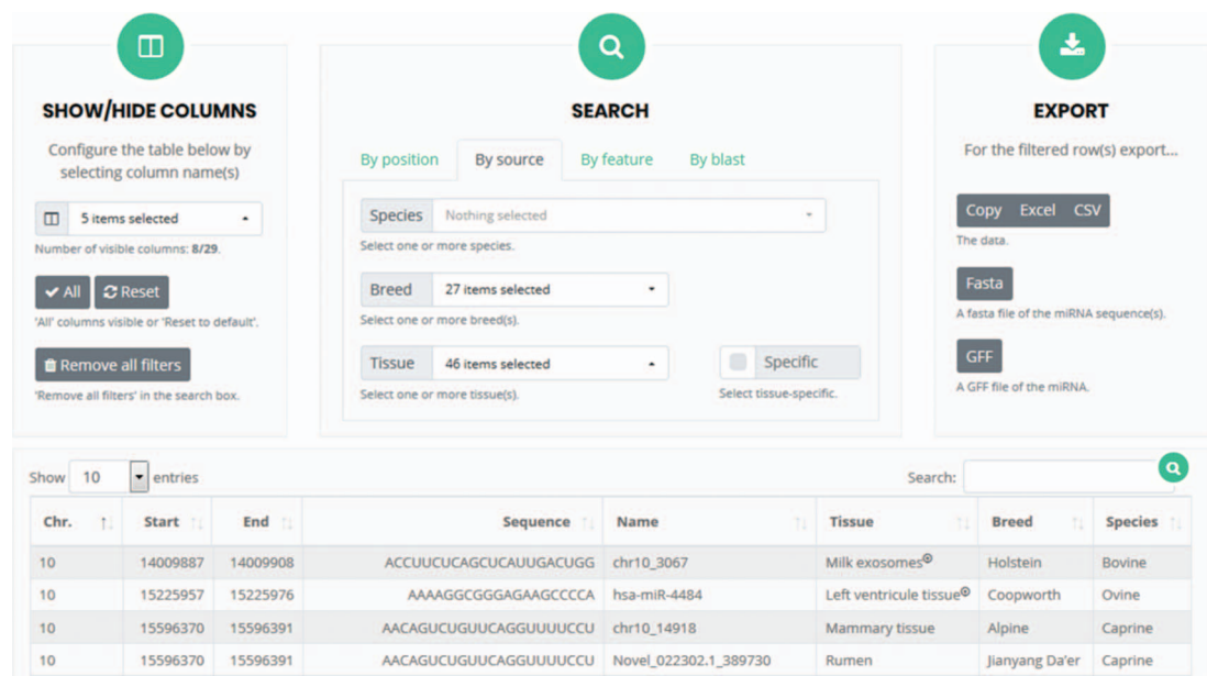
Figure 7. User interface for ‘search and browse’. Columns can be selected so that only specific features will be visible. The search box allows the detection of microRNAs present in the RumimiR database as a function of the selected choices. The results can be exported in different formats, such as Excel or Fasta.
