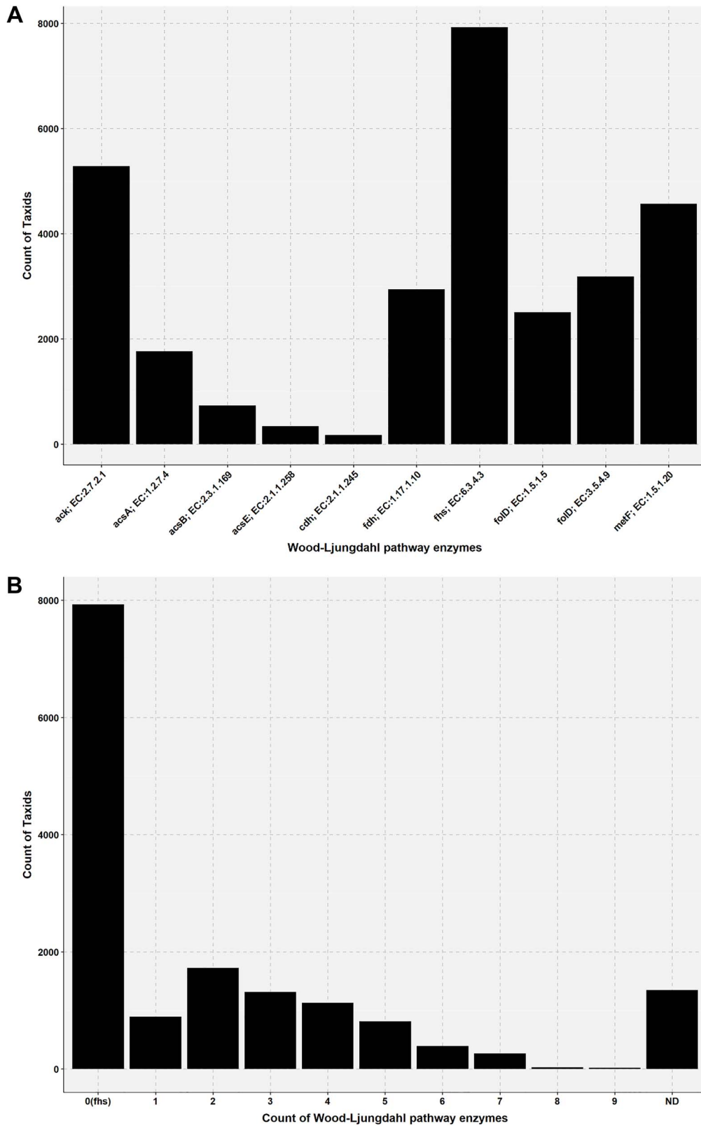
Figure 5. Bar plot showing the presence of Wood-Ljungdahl pathway enzymes in the genome of AcetoBas accessions. (A) Count of taxids for the Wood-Ljungdahl pathway enzymes in the genome of AcetoBase accessions (ND, not determined). (B) Count of taxids for the presence of particular enzymes in the Wood-Ljungdahl pathway.
